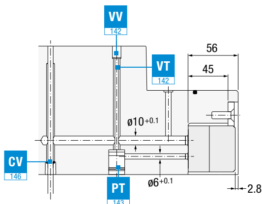
Vacuum Section
