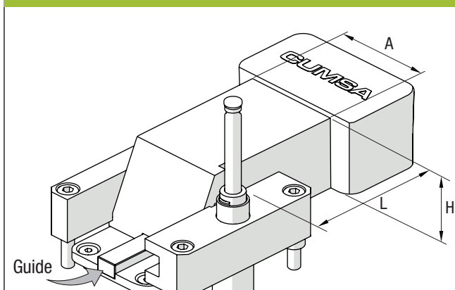
1 Unit + Guide 1.5 \times L < A < 2 \times L
